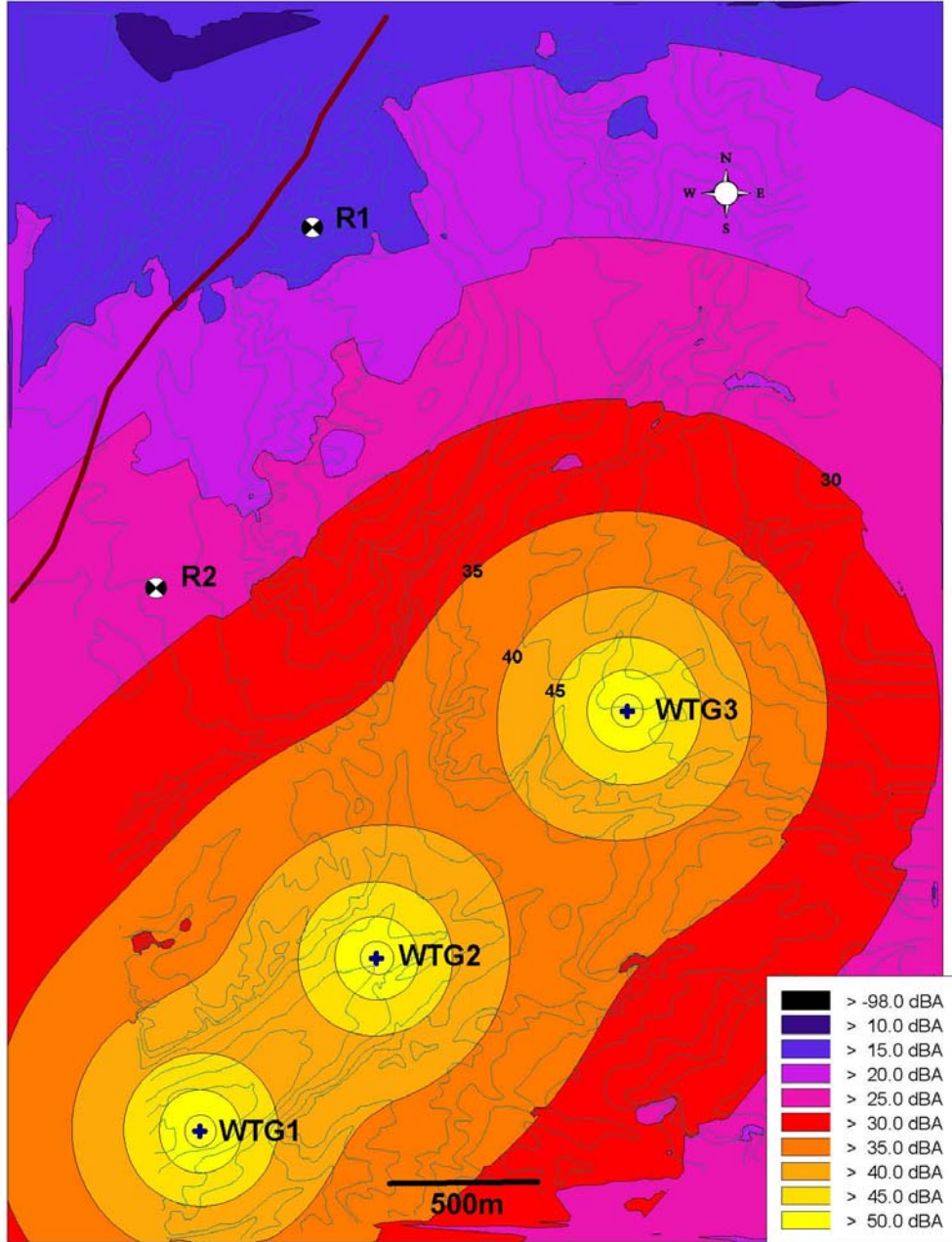
Figure 4: Representative Acoustic Model showing the Propagation of Sound from Typical Wind Turbine Generators
